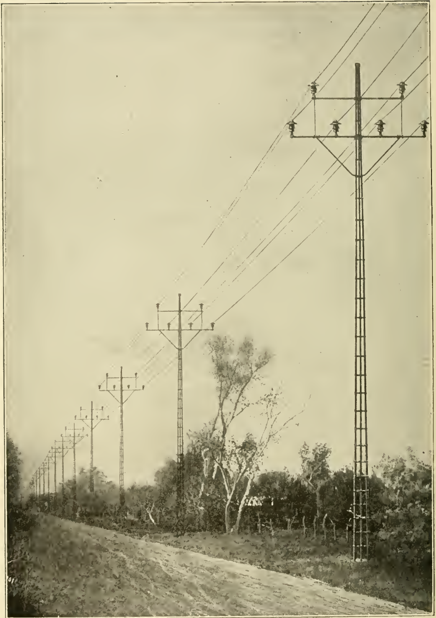
Fig. 173. Steel Pole Construction for High-Tension Circuit
